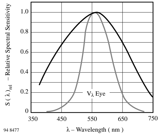
Figure 5. Relative Spectral Sensitivity vs. Wavelength
